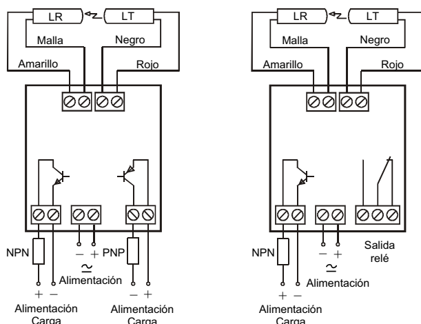
PA 11 D/E 40X Salida Transistor
