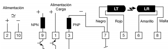
Salida Transistor – PA 11 A/B 40XT
