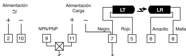
Salida Transistor – PA 10 A/B 61X
